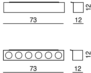
Vaschette / Storage unit
