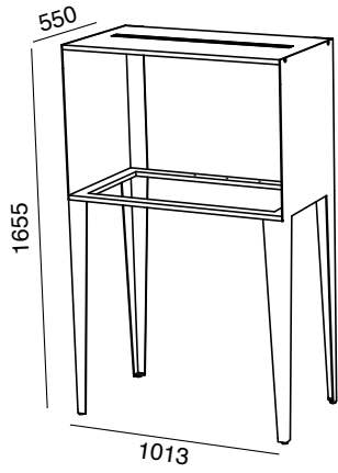
FINITURE / FINISHINGS (B) (C) (H)
